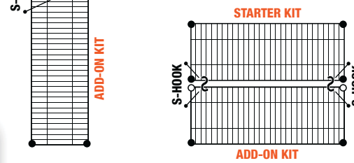
WIRE SHELVING ADD-ON LAYOUT OPTIONS
